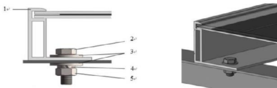
Fig.5-3 Double-glass module with frame 图 5-3 有框双玻组件安装图示
